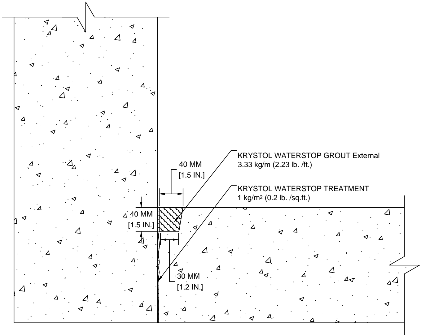
NEW CONSTRUCTION - WALL TO SLAB - (WALL INBOARD OF SLAB) REFER TO APPLICATION INSTRUCTION 4.12
